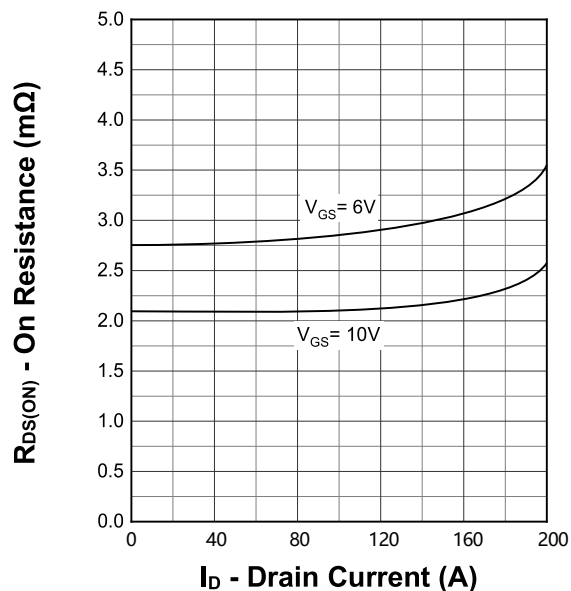
On Resistance
