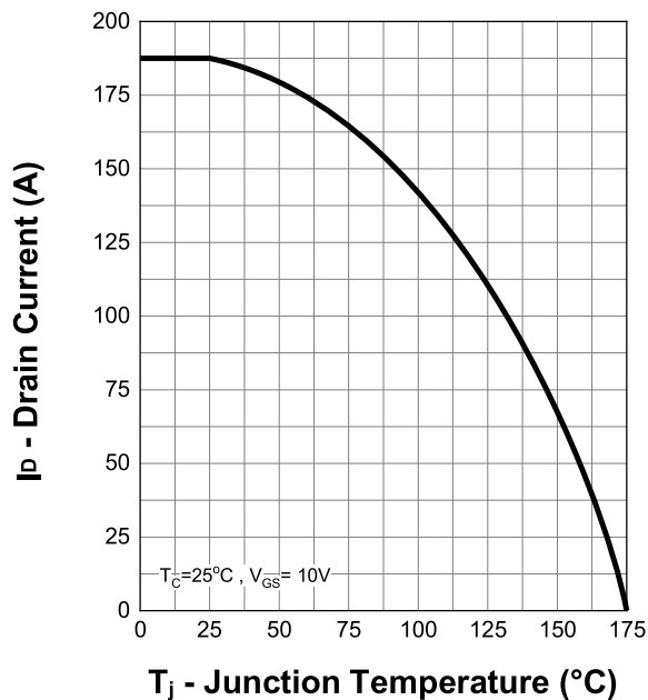
Current Capability
