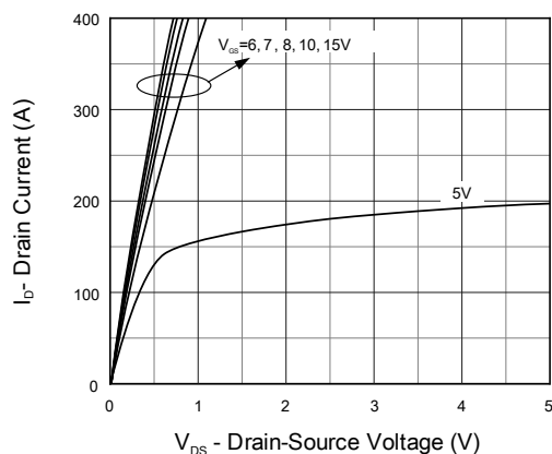
Figure 5. Output Characteristics
