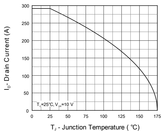
Figure 2. Current Capability
