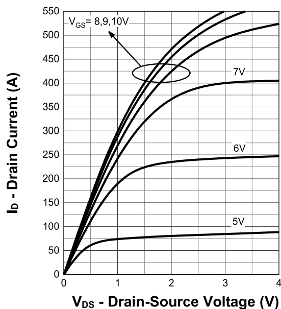
Output Characteristics
