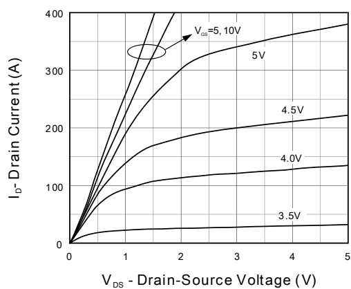
Figure 5. Output Characteristics
