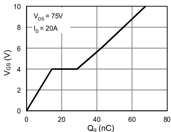
Figure 12. Gate charge
