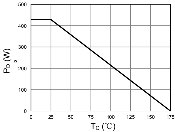
Figure 1. Power Capability
