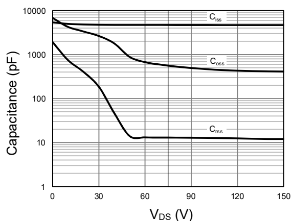
Figure 11. Capacitance
