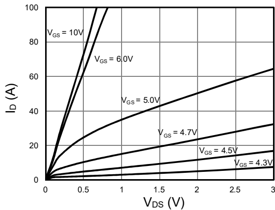
Figure 3. Output characteristics
