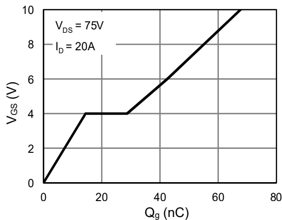
Figure 12. Gate charge
