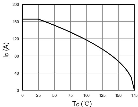
Figure 2. Current Capability
