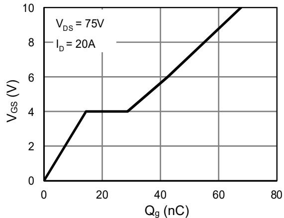
Figure 12. Gate charge
