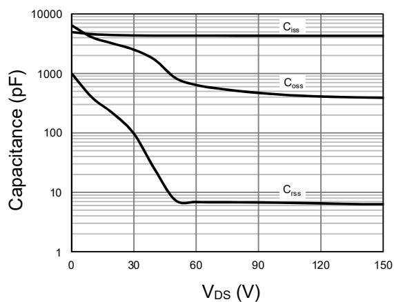
Figure 11. Capacitance
