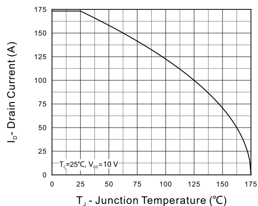
Figure 2. Current Capability
