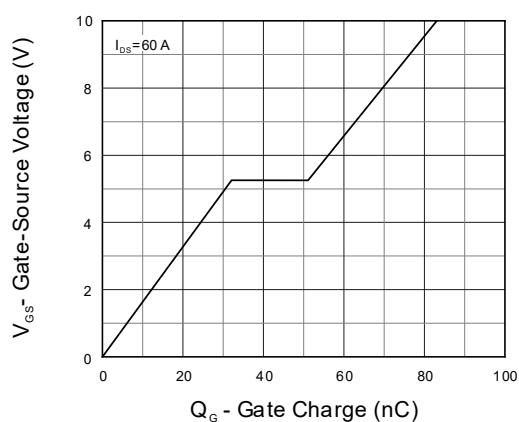
Figure 12. Gate Charge
