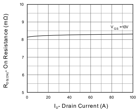
Figure 6. On Resistance
