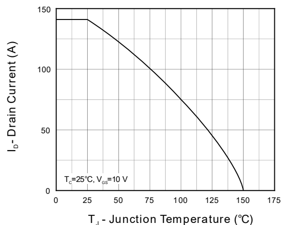
Figure 2. Current Capability
