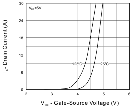
Figure 7. Transfer Characteristics
