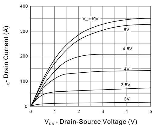
Figure 5. Output Characteristics
