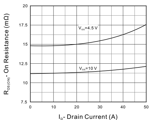
Figure 6. On Resistance
