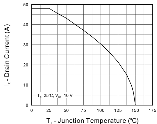
Figure 2. Current Capability
