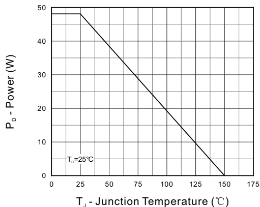
Figure 1. Power Capability
