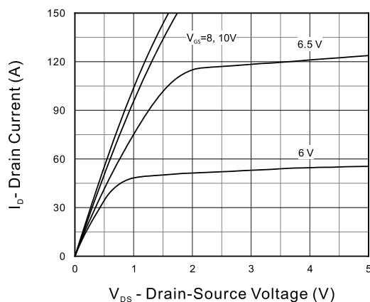
Figure 5. Output Characteristics
