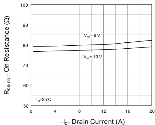
Figure 6. R_{DS(ON)} vs. I_D
