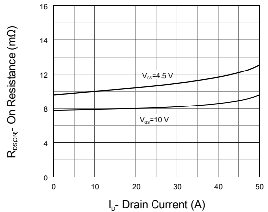
Figure 6. On Resistance
