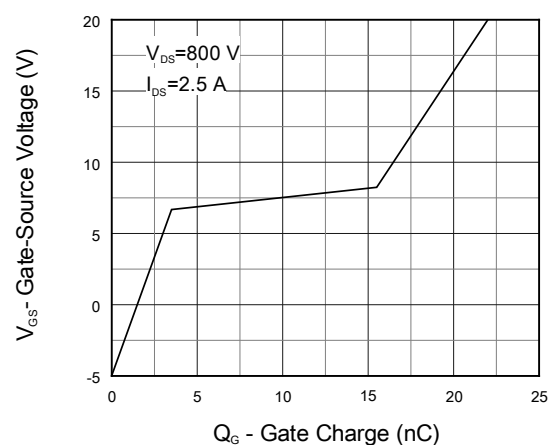
Fig 12. Gate Charge
