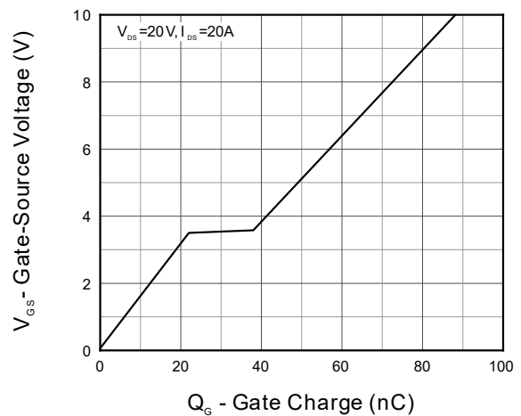
Figure 12. Gate Charge
