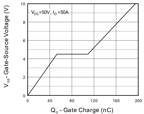
Figure 12. Gate Charge
