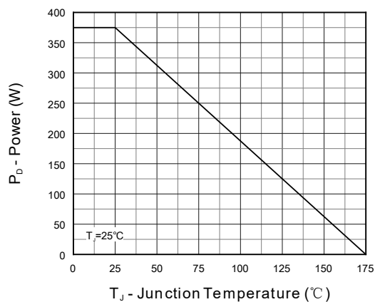
Figure 1. Power Capability
