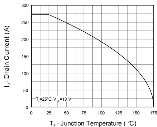
Figure 2. Current Capability
