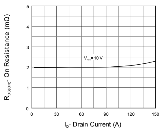
Figure 6. On Resistance
