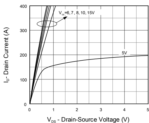
Figure 5. Output Characteristics
