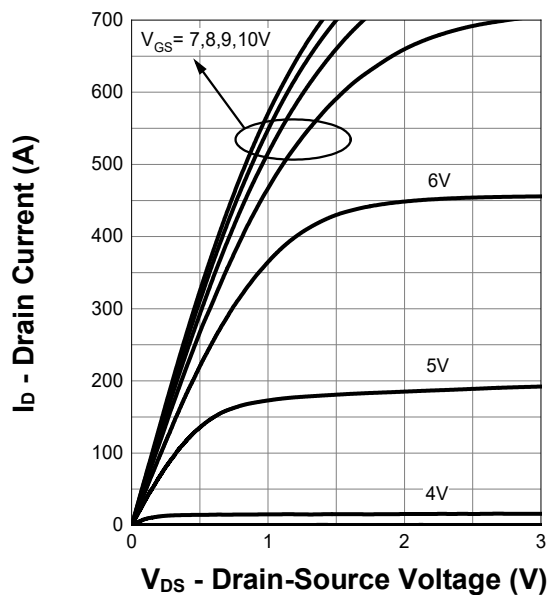
Output Characteristics
