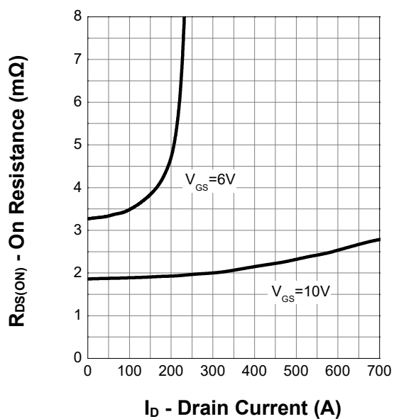
On Resistance
