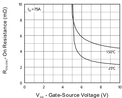
Figure 7. Transfer Characteristics
