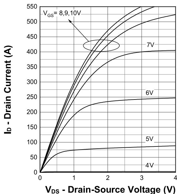
Output Characteristics
