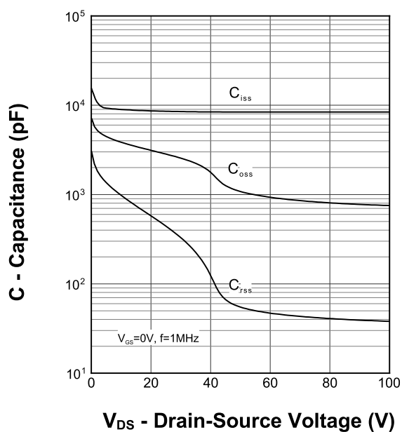
Capacitance
