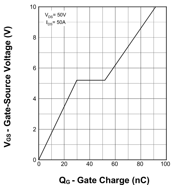
Gate Charge
