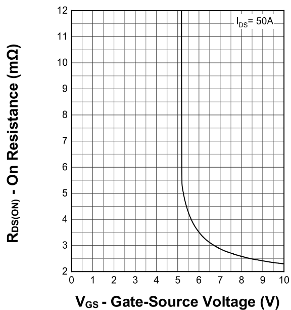
Transfer Characteristics
