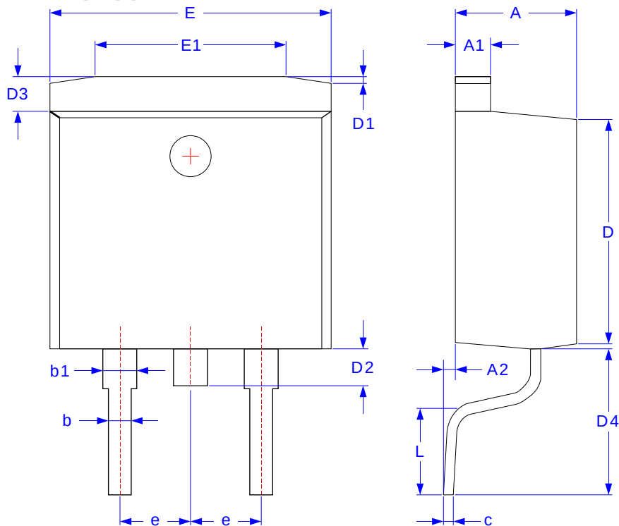
TO-263 Package (1)
