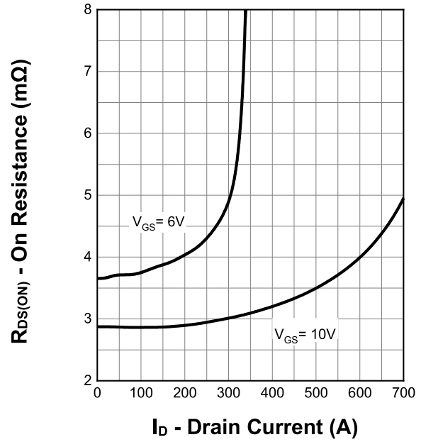
On Resistance
