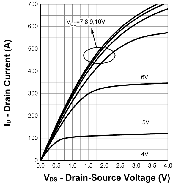
Output Characteristics
