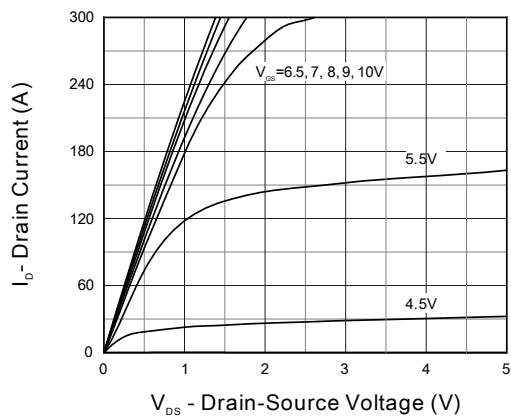
Figure 5. Output Characteristics
