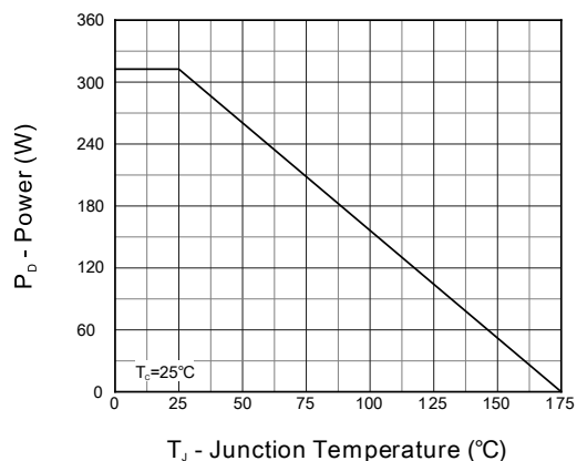
Figure 1. Power Capability
