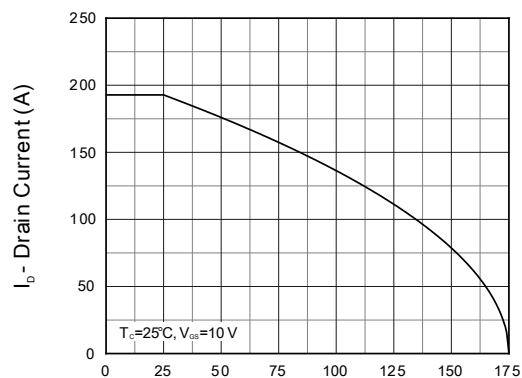
Figure 2. Current Capability
