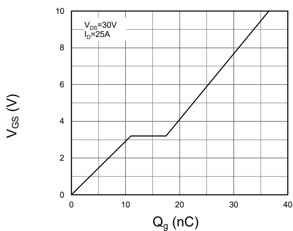
Fig 11. Gate charge
