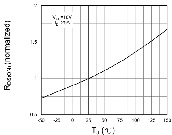
Fig 7. On-resistance vs T_J
