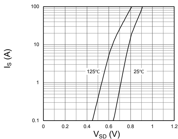
Fig 9. Forward Characteristics of Body Diode
