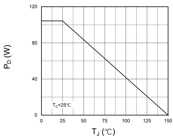
Fig 1. Power capability
