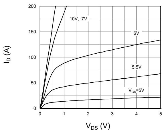
Fig 5. Output characteristics
