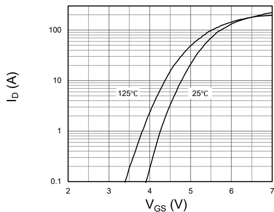
Fig 8. Typical Transfer Characteristics
