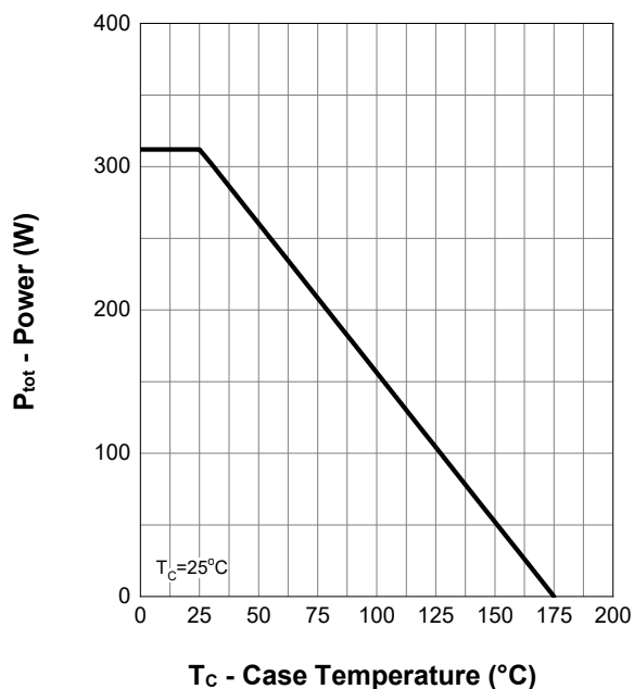
Power Capability
