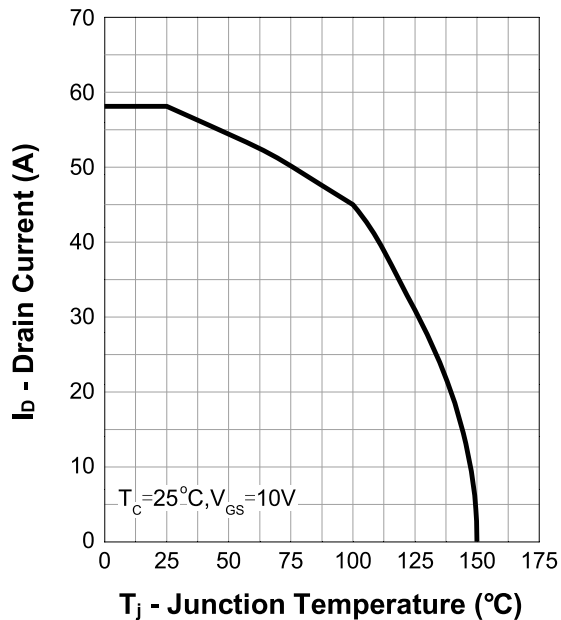
Current Capability
