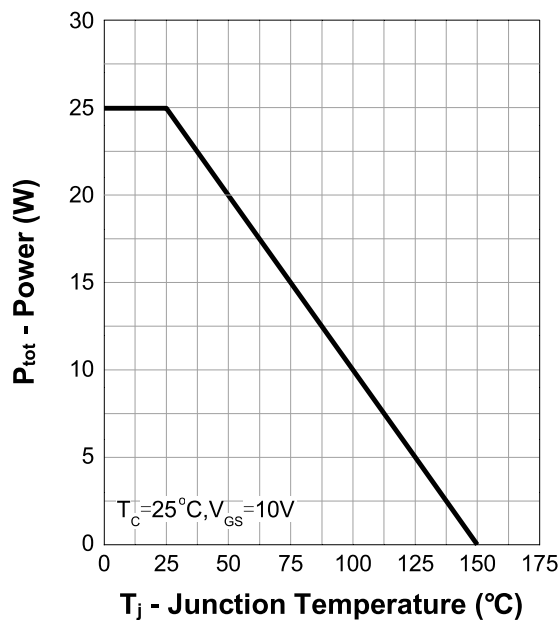
Power Capability
