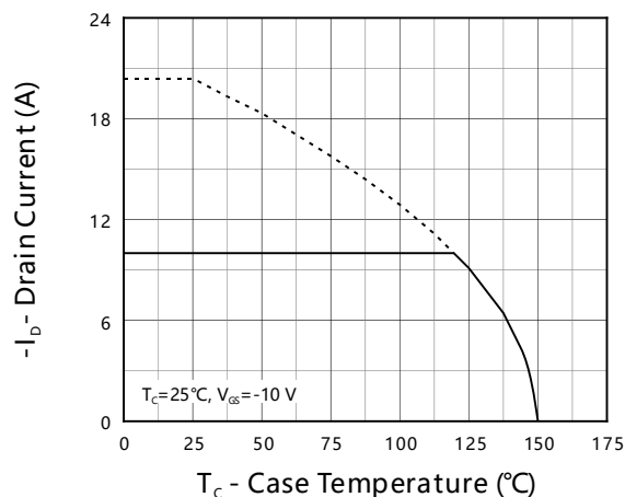
Fig 2. Current Capability
