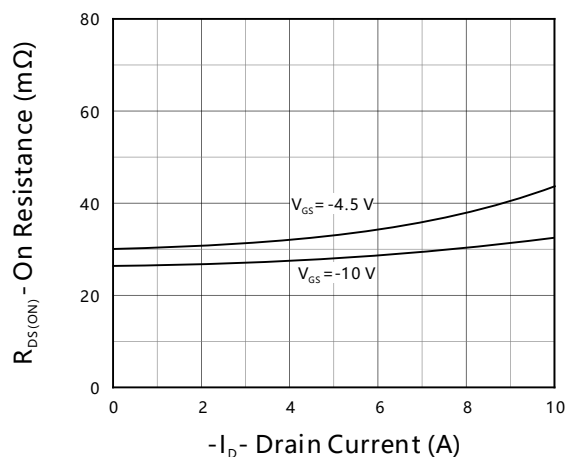
Fig 6. On Resistance
