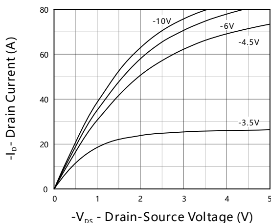
Fig 5. Output Characteristics
