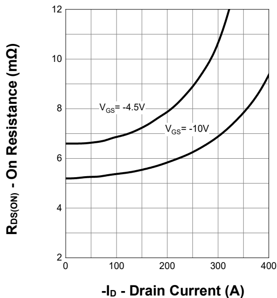
On Resistance
