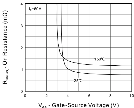
Fig 7. Transfer Characteristics
