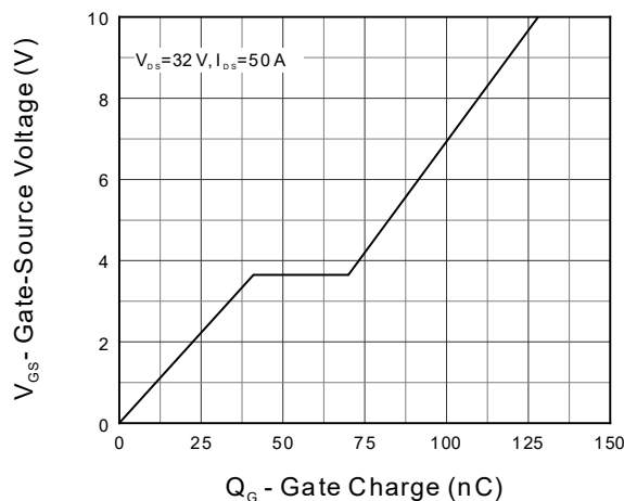
Fig 12. Gate Charge
