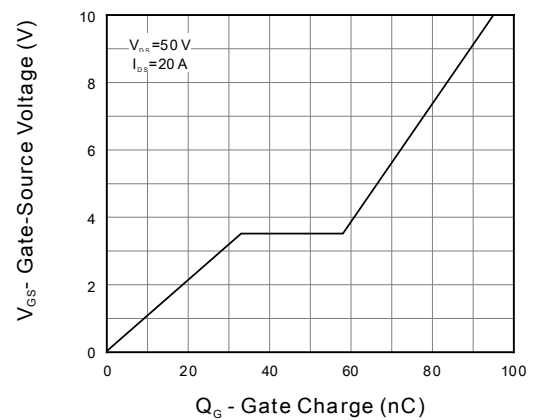
Figure 12. Gate Charge
