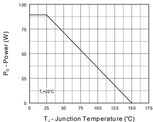
Figure 1. Power Capability
