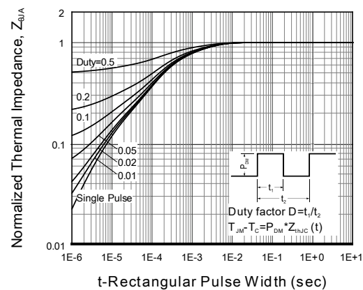
Figure 4. Normalized Maximum Transient Thermal Impedance
