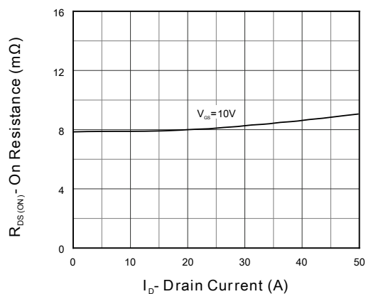
Figure 6. On Resistance
